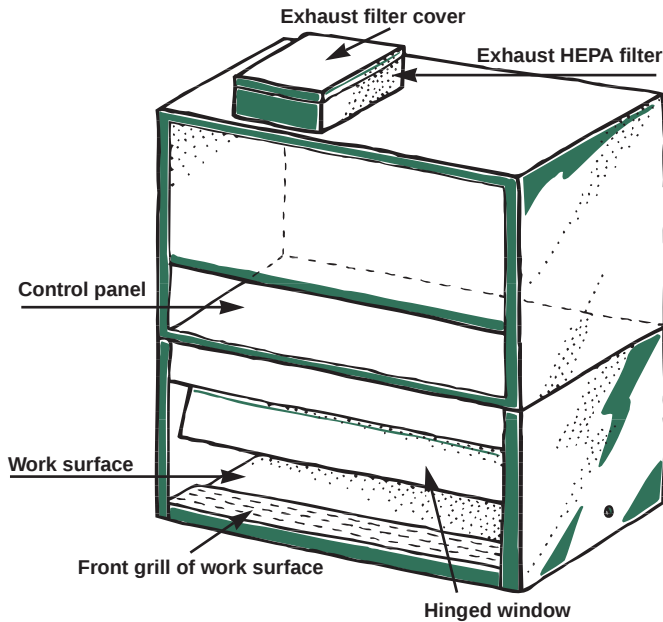
Figure 3. Class I biological safety cabinet
