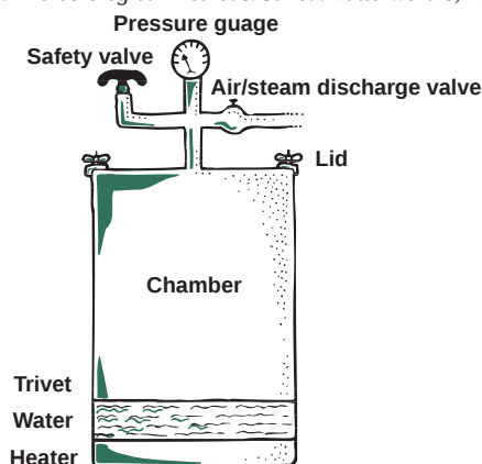
Figure 6. Pressure cooker laboratory autoclave
