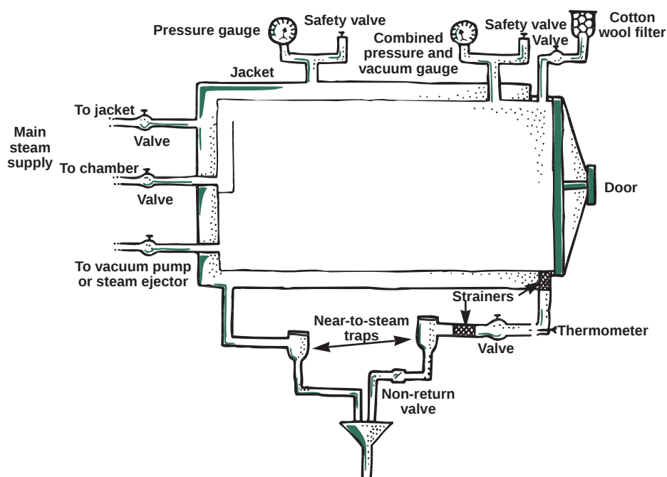
Figure 7. Autoclave with air discharge by gravity displacement
